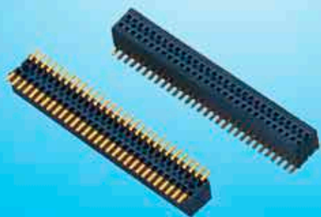
1.27mm Female Header
