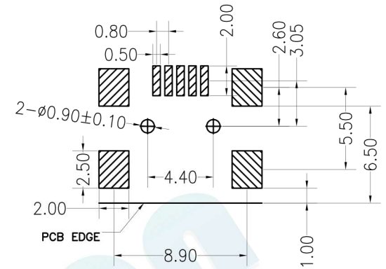
RECOMMENDED P.C.B. PATTERN LAYOUT
