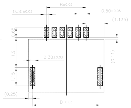
RECOMMEND PCB LAYOUT TOLERANCE: ±0.05
